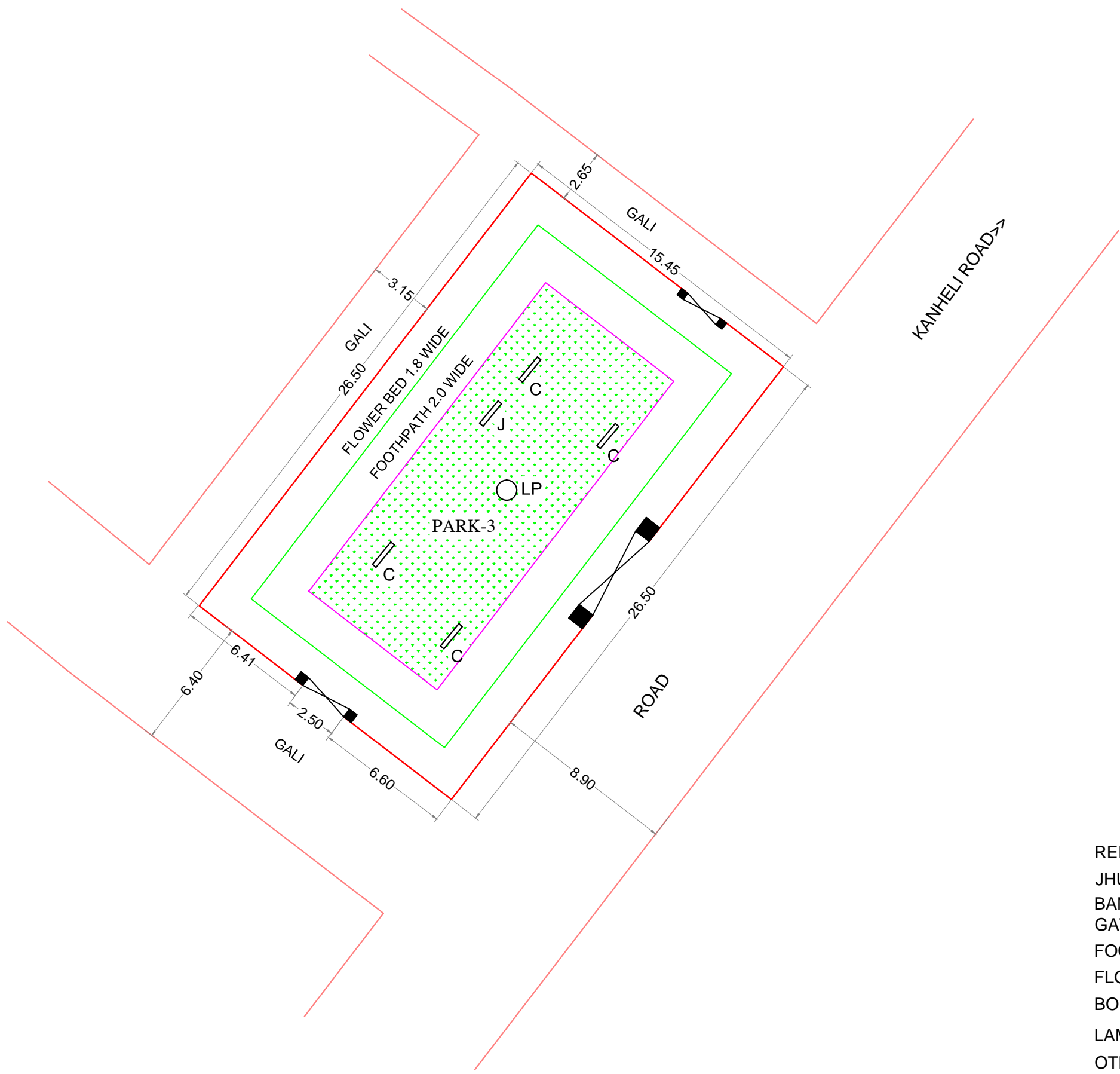
LOCATION PLAN
